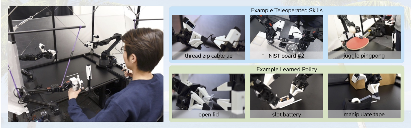
Fig. 1: ALOHA 🍷: A L ow-cost O pen-source H ardware System for Bimanual Teleoperation. The whole system costs <$20k with off-the-shelf robots and 3D printed components. Left : The user teleoperates by backdriving the leader robots, with the follower robots mirroring the motion. Right : ALOHA is capable of precise, contact-rich, and dynamic tasks. We show examples of both teleoperated and learned skills.
